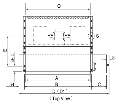
Figure 3 : HCCA Unit With Bottom Return Plenum
